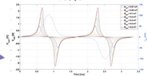
Figure3: simulated excitation current and raw output signal
