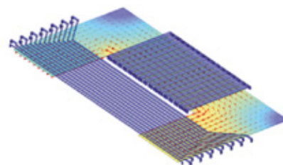
Figure2: FEM analysis of a miniaturized fluxgate sensor
