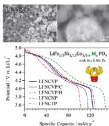
Figure 1 - Morphology and battery performance of advanced high-voltage cathodes for LIBs
