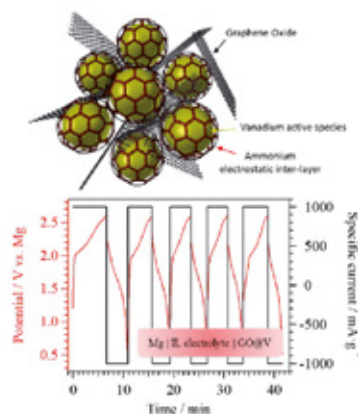
Figure 2 - Architecture and performance of an advanced cathode material for magnesium secondary batteries
