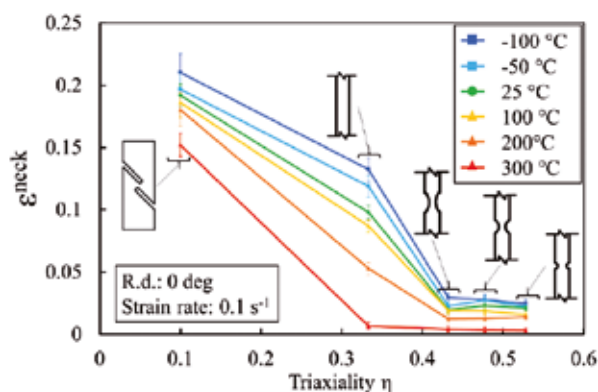
Fig.2 : Necking locus at varying temperautre.
