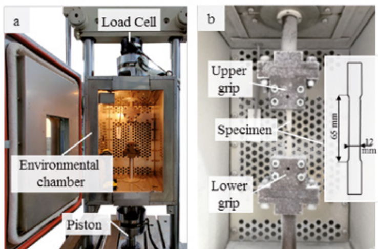
Fig.1 : Experimental equipment for sub-zero temperature tests.
